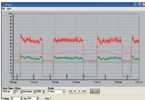
Above: CMS download graph showing power draw, hydraulic pressure, crusher setting and ancillary inputs.
